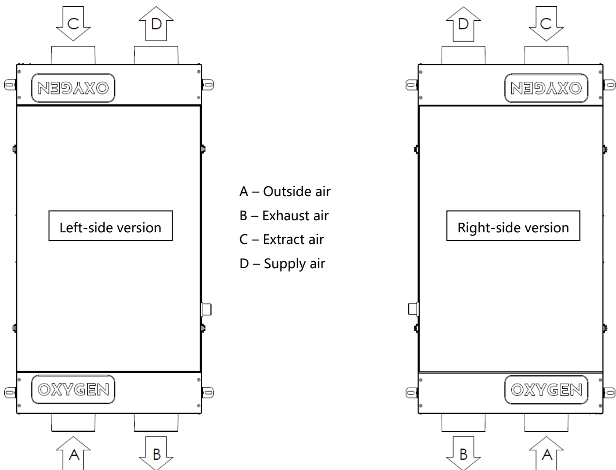
Figure 2. Mounting orientation
