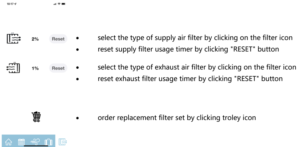
Figure 18. Filter menu
