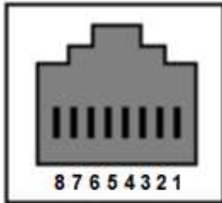
Figure 7. Contacts of functions connector
