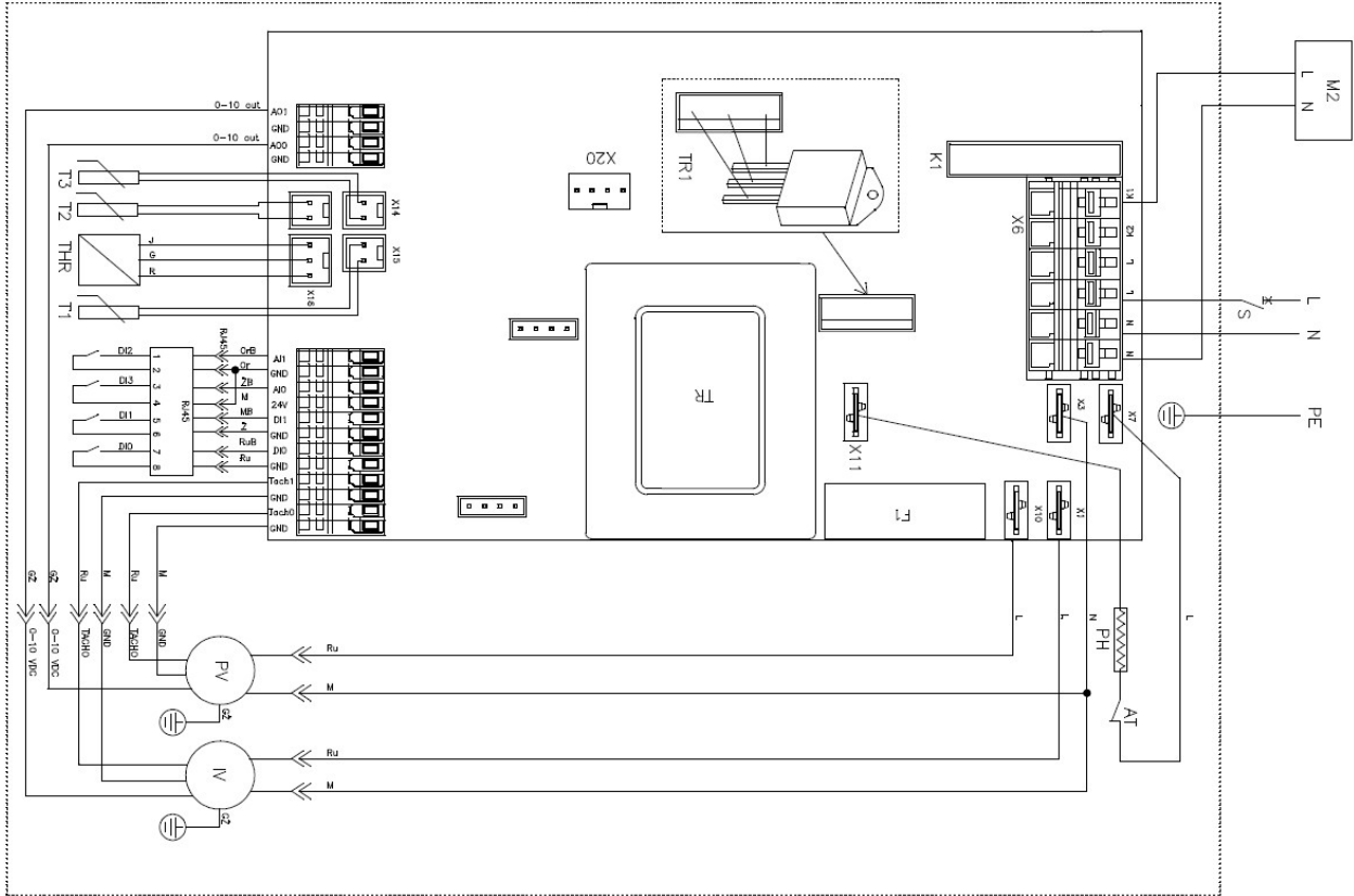
Figure 9. Control board electrical wiring diagram
