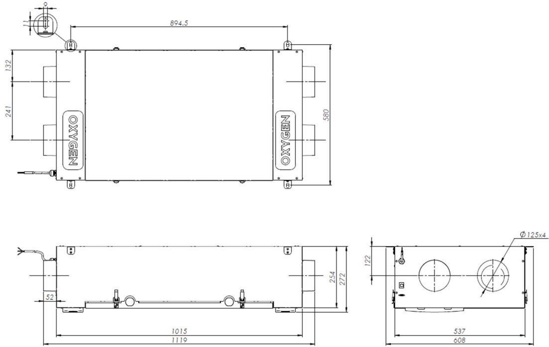
Figure 1. Unit dimensions
