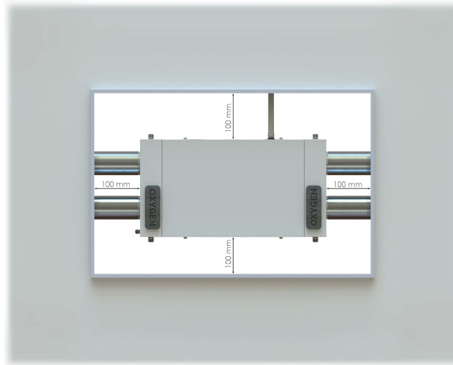
Figure 4. Installation of maintenance and service hatch
