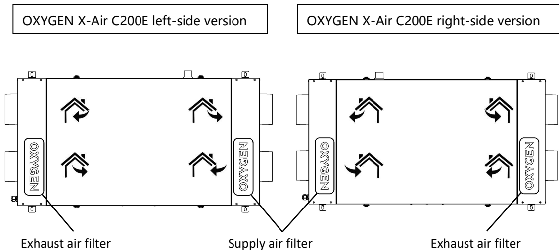
Figure 27. Locating air filters
