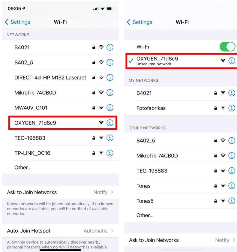
Figure 11. WiFi connection set-up
