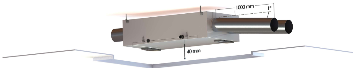
Figure 3. Air intake duct connection diagram
