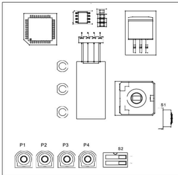
Figure 26. Additional settings for control panel with a knob
