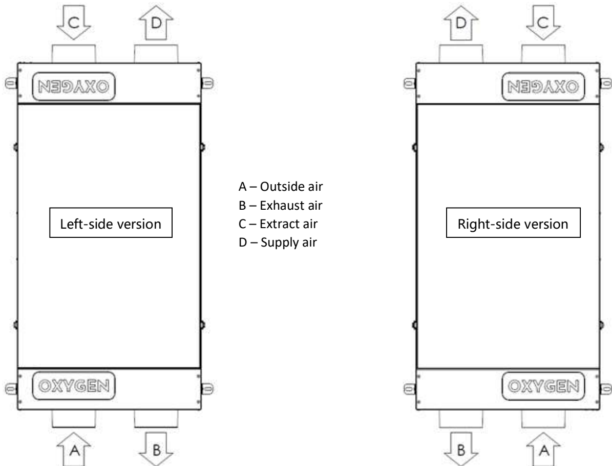
Figure 2. Mounting orientation
