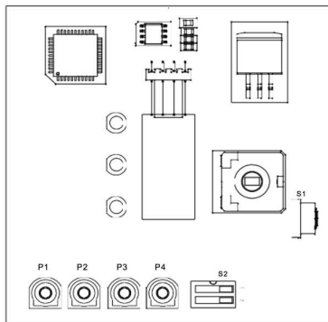
Figure 29. Additional settings for control panel with a knob
