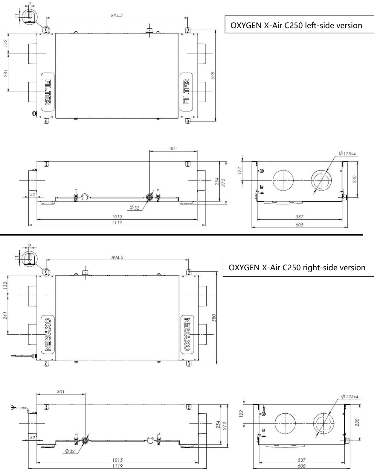
Figure 1. Unit dimensions
