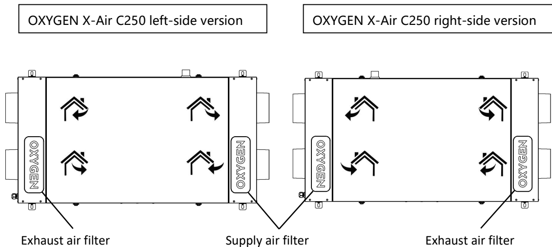
Figure 30. Locating air filters
