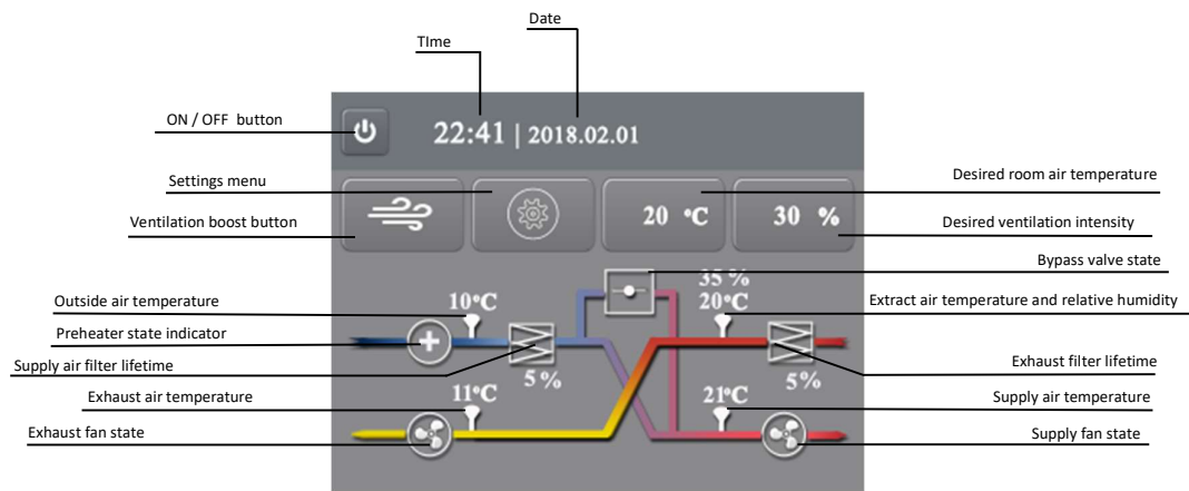
Figure 23. Main screen of control panel with touchscreen display
