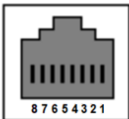
Figure 6. Contacts of functions connector
