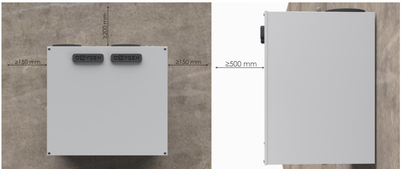
Figure 3. Maintenance space
