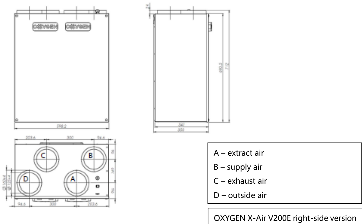
Figure 1. Unit dimensions
