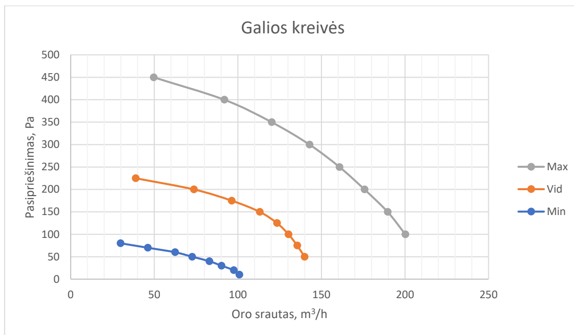
Graph. 1. Ventilation power dependence on the resistance of installed ventilation system
