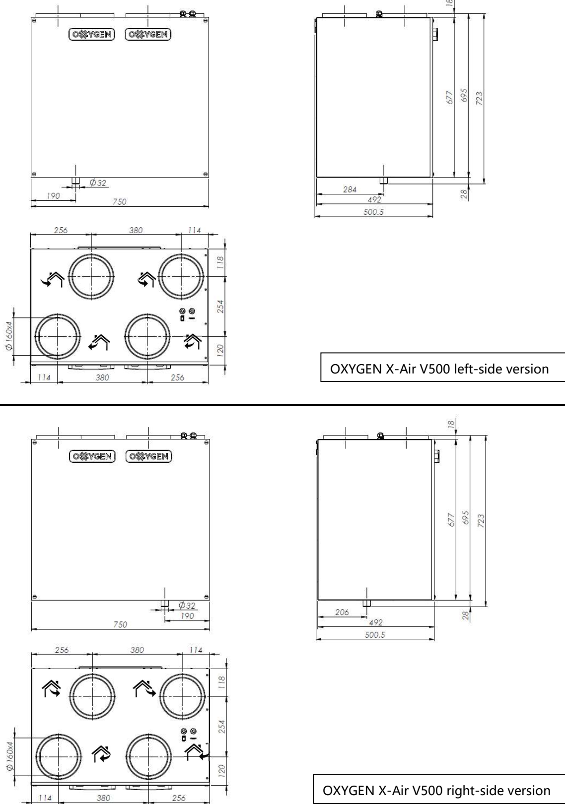
Figure 1. Unit dimensions
