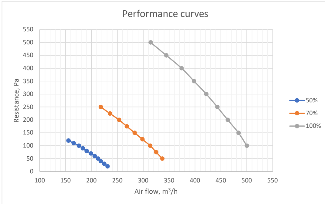
Graph. 1. Ventilation power dependence on the resistance of installed ventilation system
