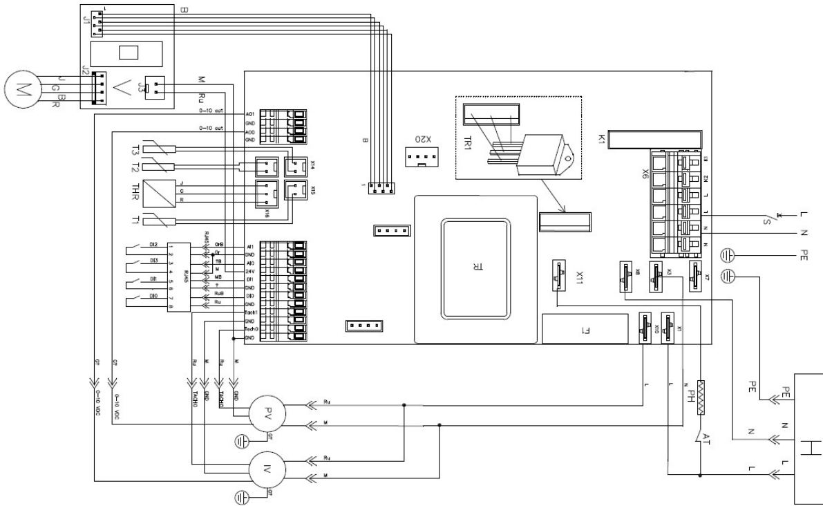
Figure 10. Control board electrical wiring diagram
