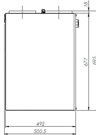
OXYGEN X-Air V400E left-side version
