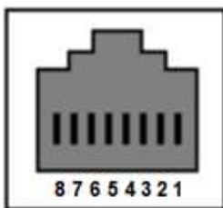
Figure 6. Contacts of functions connector
