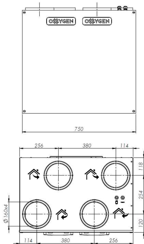
Figure 1. Unit dimensions
