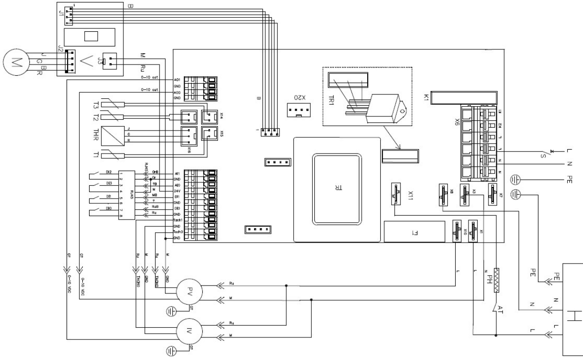
Figure 8. Control board electrical wiring diagram
